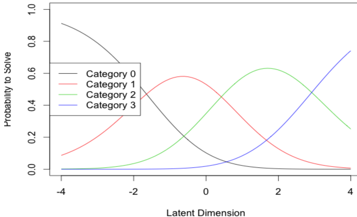
ICC plot for item simp1
